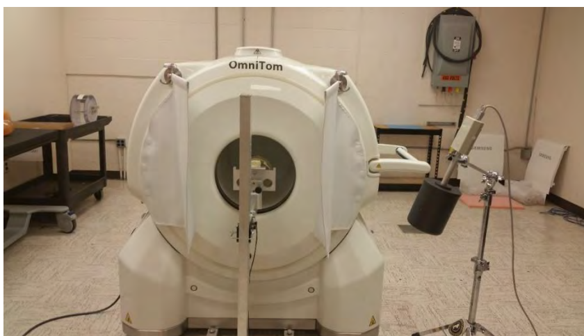
Figure 157: The scatter measurement setup
