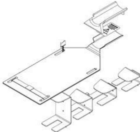
Figure 271: Universal transfer board and stiffeners
