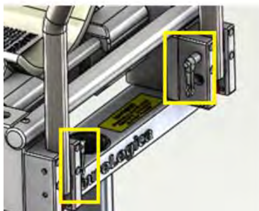
Figure 284: Locking pins for the handle
