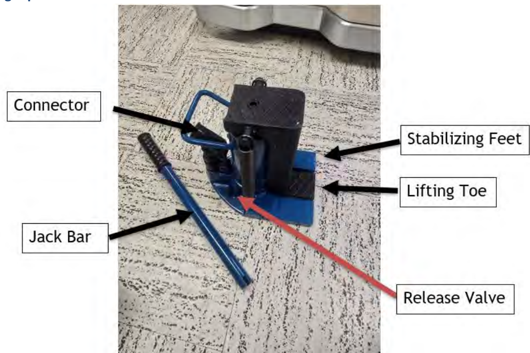
Figure 296: Jack Components
