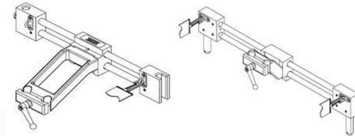
Figure 257: Bed adapter without posts (left) and bed adapter with posts (right)
