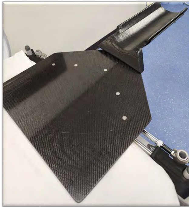
Figure 262: Silhouette scan board attached to bed adapter
