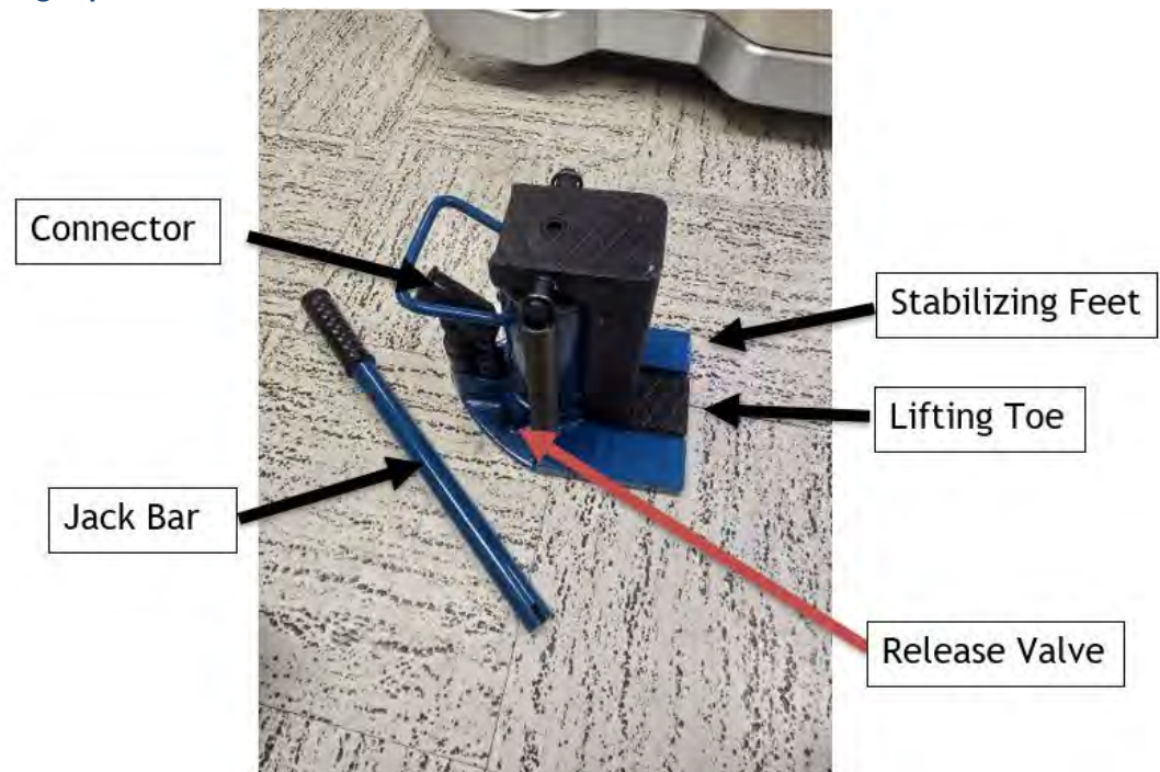
Figure 288: Jack Components
