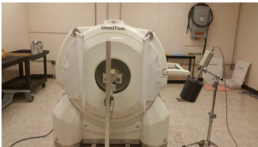
Figure 151: The scatter measurement setup
