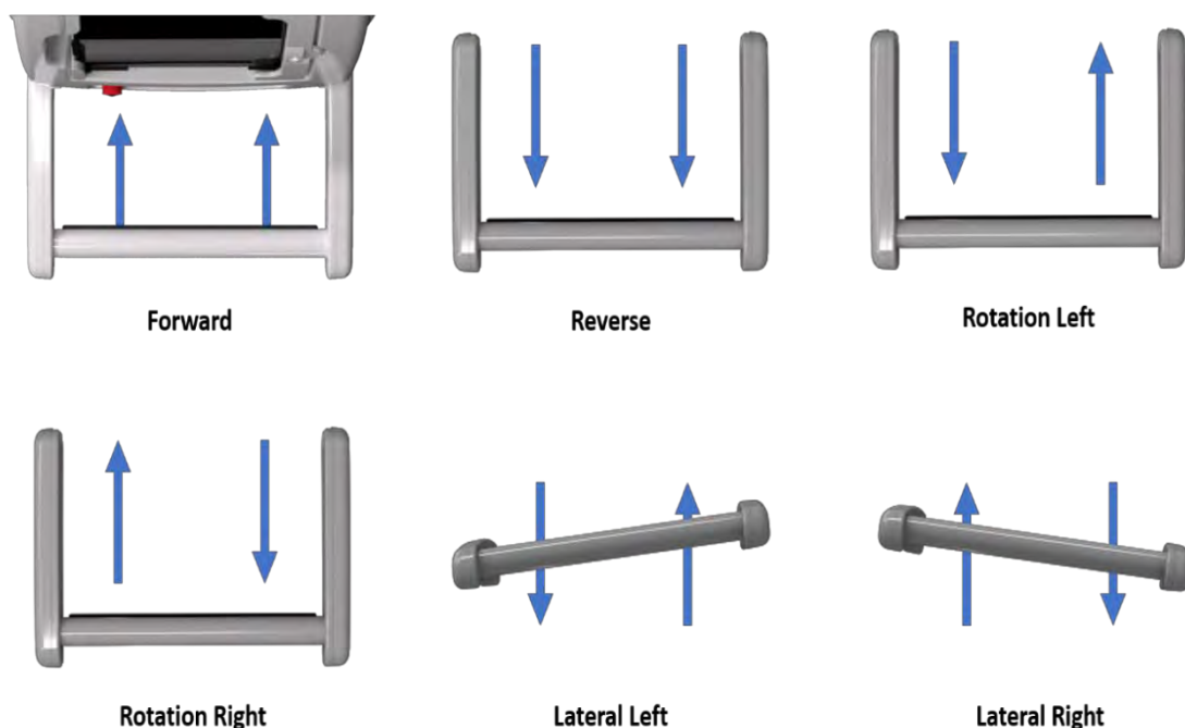
Figure 18: Drive bar motions
