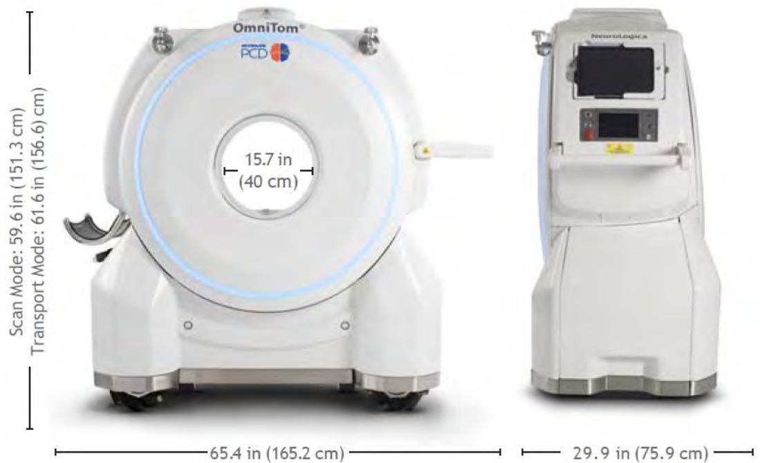
Figure 1: Scanner dimensions
