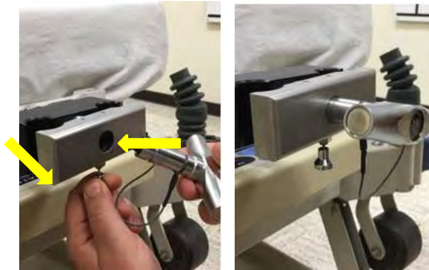
Figure 262: Steps showing reattaching T-square handle
