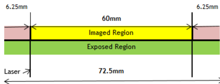
Figure 166: Scan coverage and imaged region for a true coverage of 60mm
