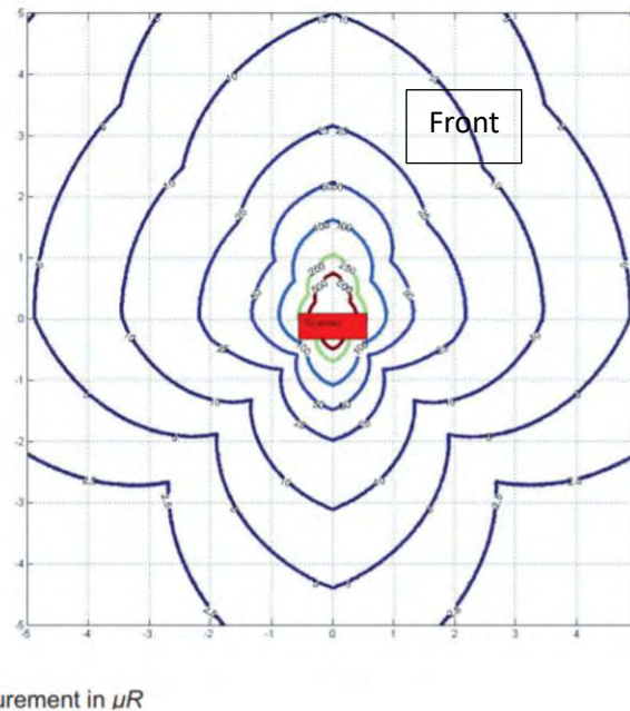
Figure 152: The isodose curves for 120 kV, 70 mAs using the CTDI 16cm phantom. The distances are in meters, and the scatter is measured in \mu R .
