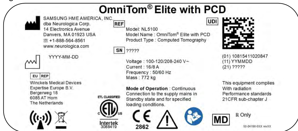
Figure 2: Product marking plate
